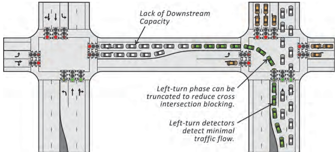
Exhibit 12-14 Phase Truncation Example
