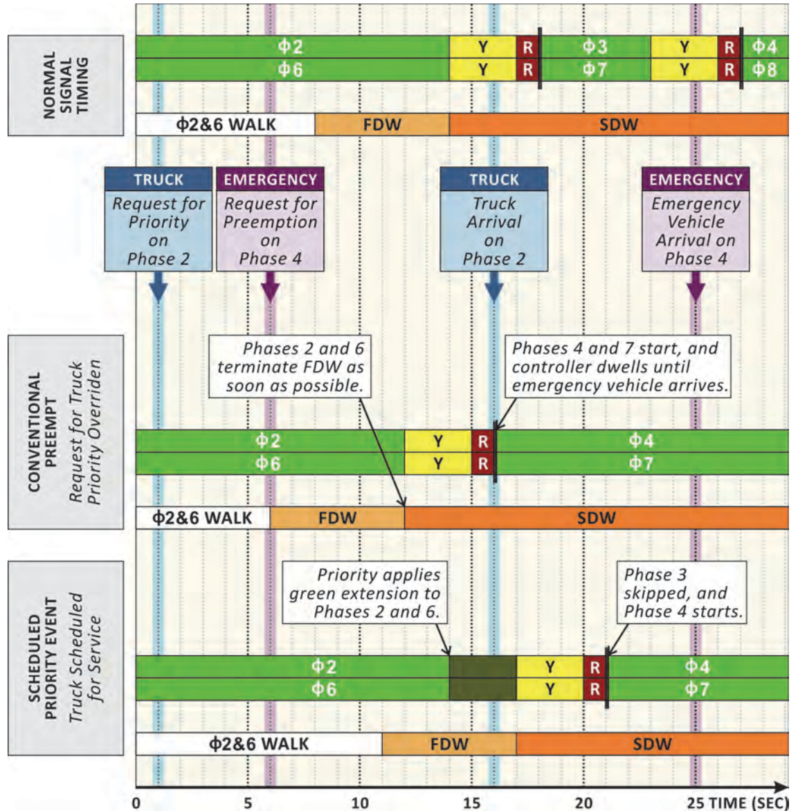
Exhibit 10-11 Accommodating Multiple Preferential Treatment Requests through Scheduling
