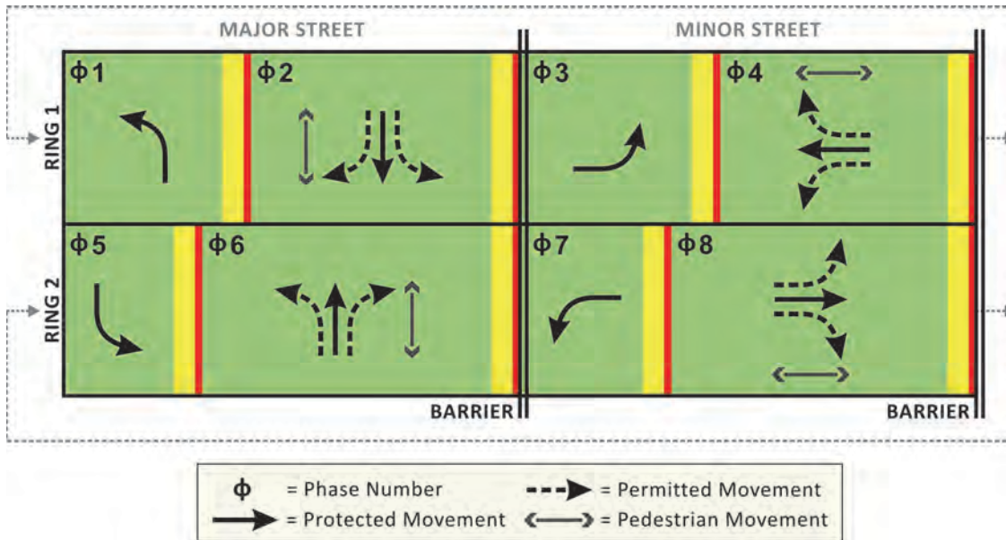
Exhibit 5-7 Ring-and-Barrier Diagram Showing Protected-Permitted Left-Turn Phasing
