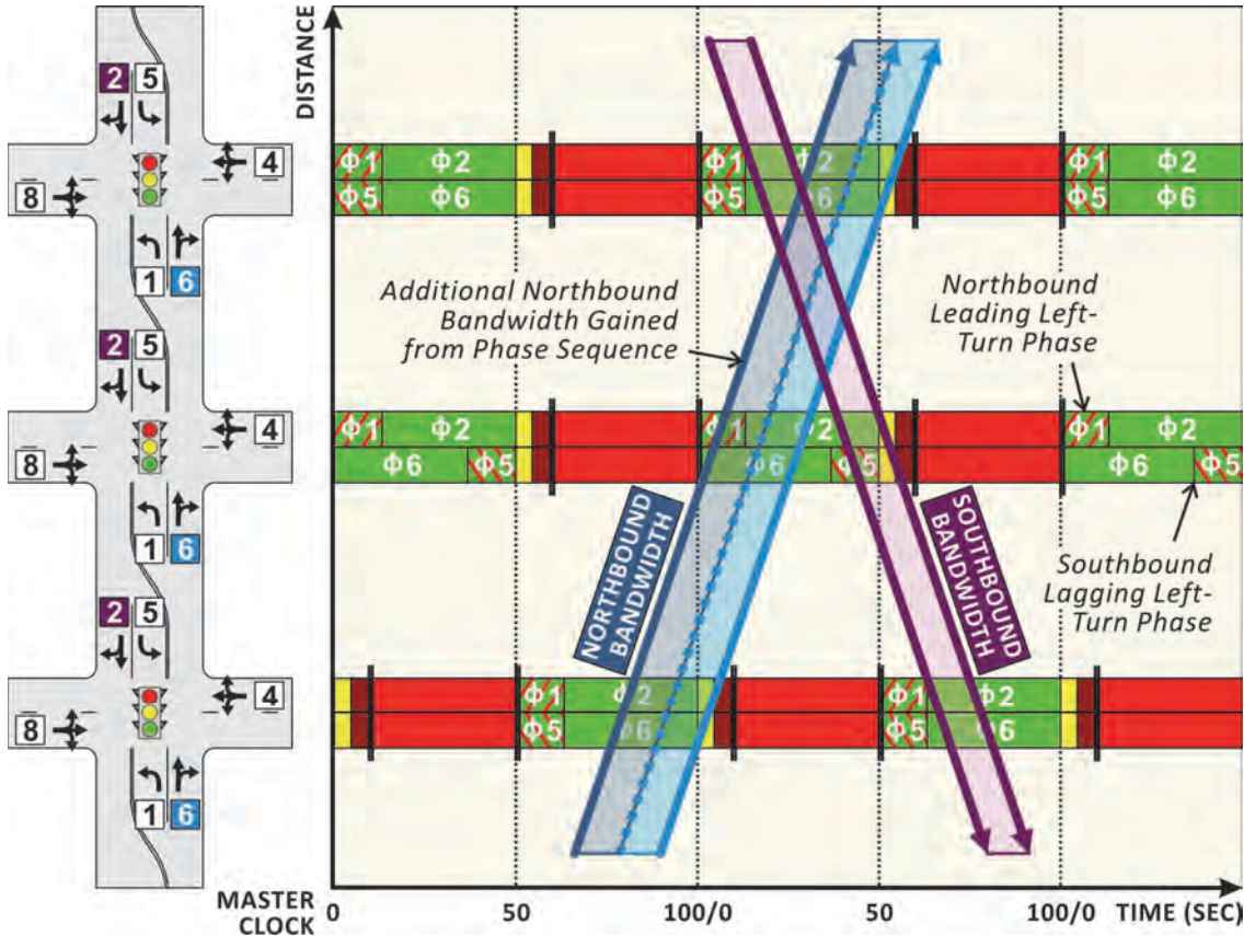
Exhibit 7-10 Phase Sequence Impacts on Bandwidth (Lead-Lag Left Turns at Middle Intersection)
