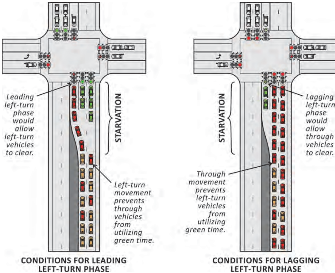
Exhibit 12-15 Conditions for Leading and Lagging Left-Turn Phases
