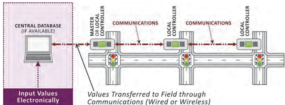
Exhibit 8-3 Signal Timing Transfer Using a Central System
