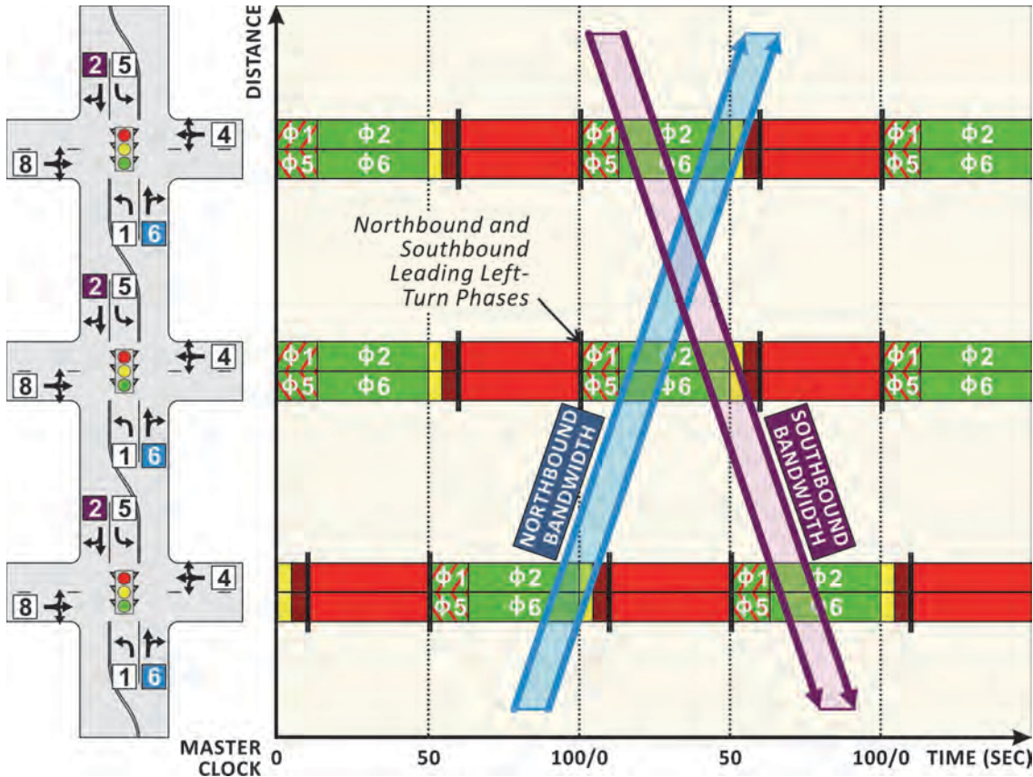
Exhibit 7-9 Phase Sequence Impacts on Bandwidth (Leading Left Turns)
