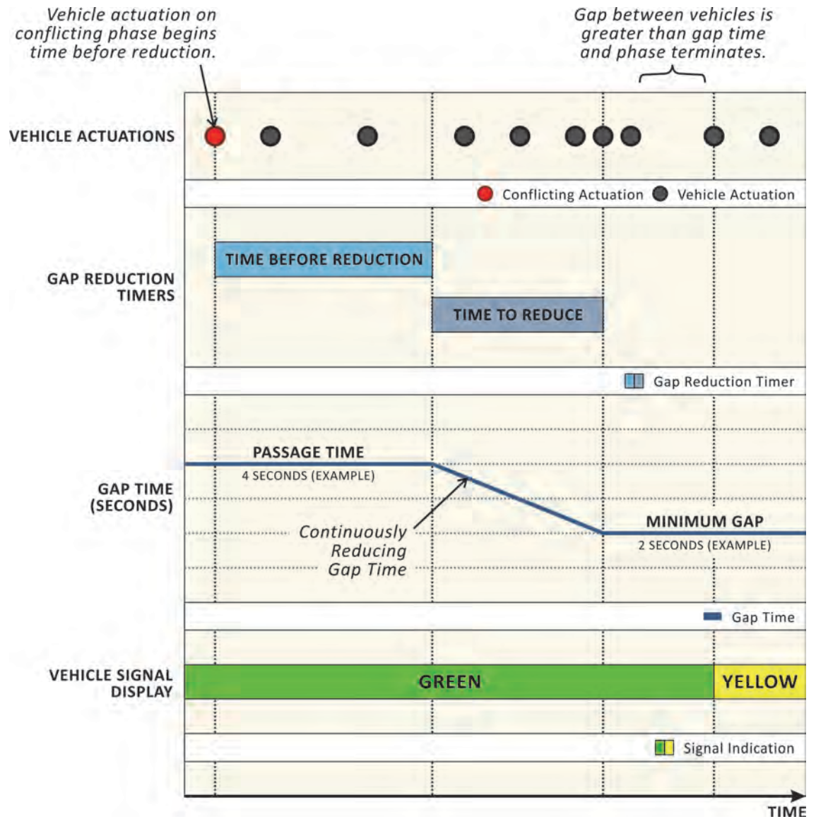
Exhibit 6-13 Relationship between Passage Time, Minimum Gap, Time before Reduction, and Time to Reduce
