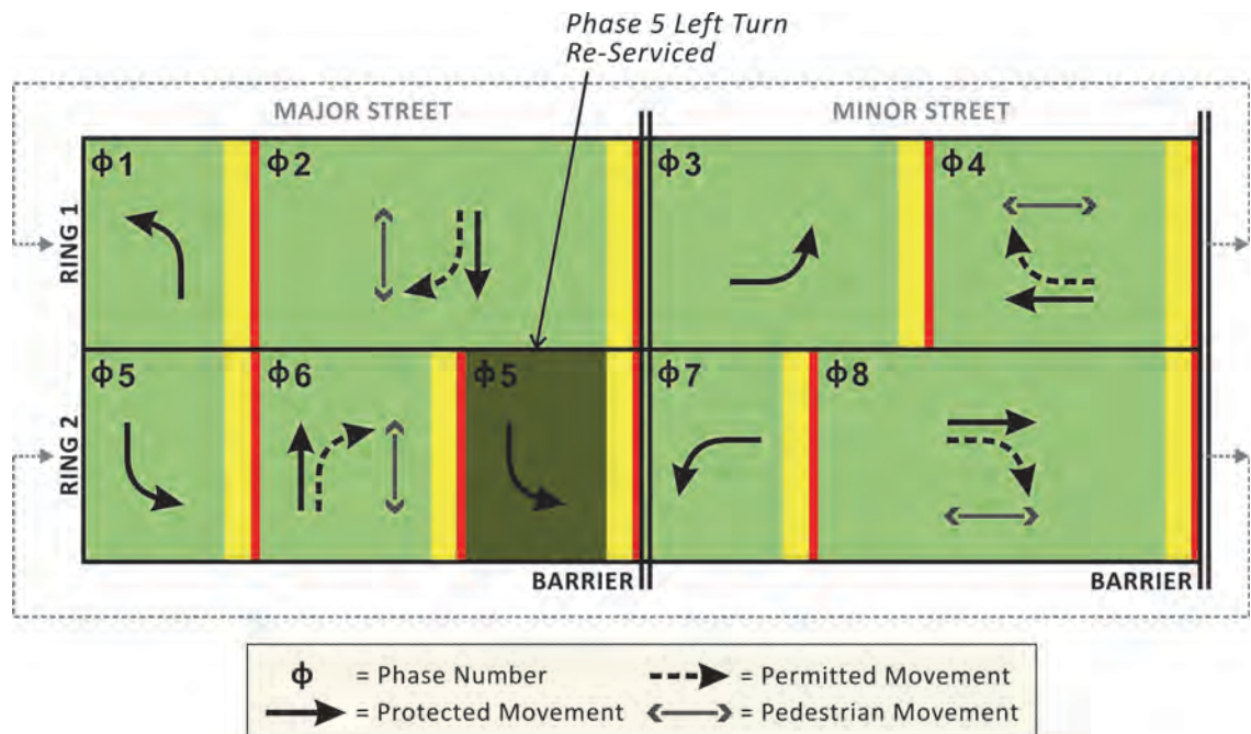
Exhibit 12-11 Ring-and-Barrier Diagram for Re- Service of Left-Turn Phase
