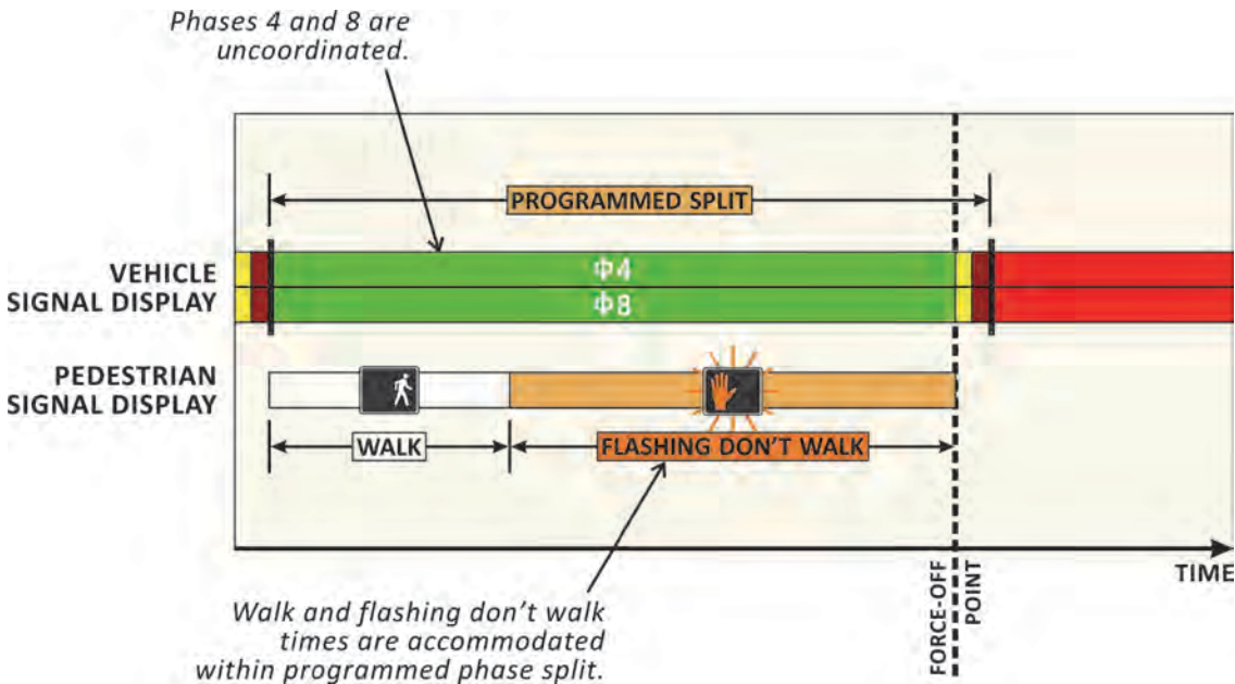
Exhibit 7-24 Uncoordinated Phase Operation with Pedestrian Timing Completed Before the Force-Off
